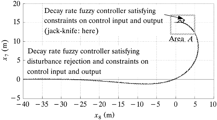
Fig. 8.6 Simulation result 4.
