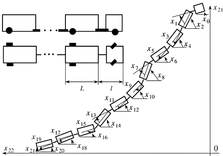
Fig. 8.12 Ten-trailer case.
