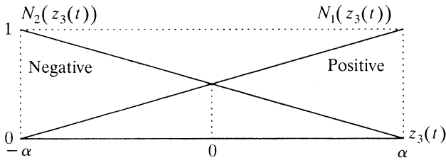
Fig. 2.9 Membership functions N_1(z_3(t)) and N_2(z_3(t)) .
